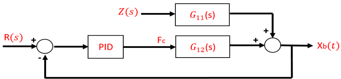
Figure 5. Closed-loop block diagram for the SI method.
