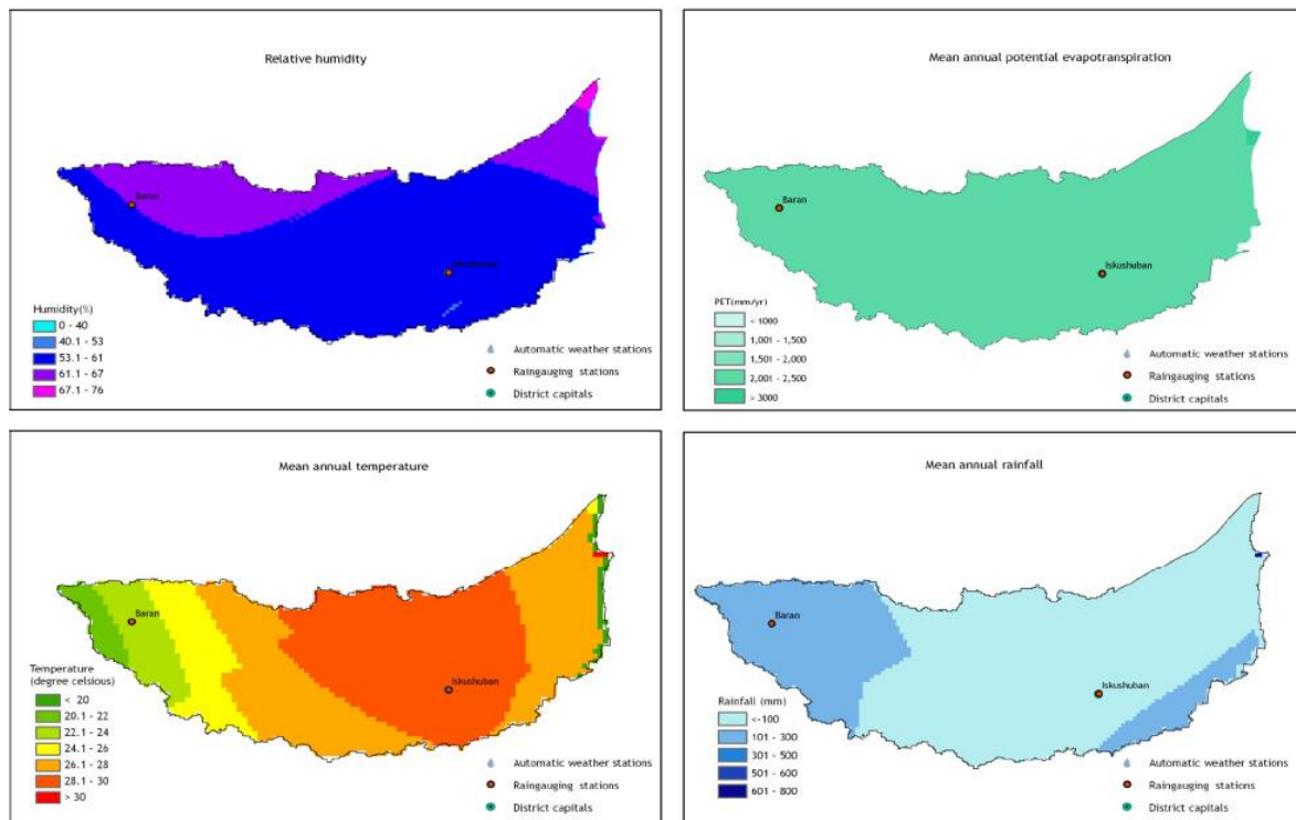
Figure 3. Mean annual weather pattern maps for Darror Basin
