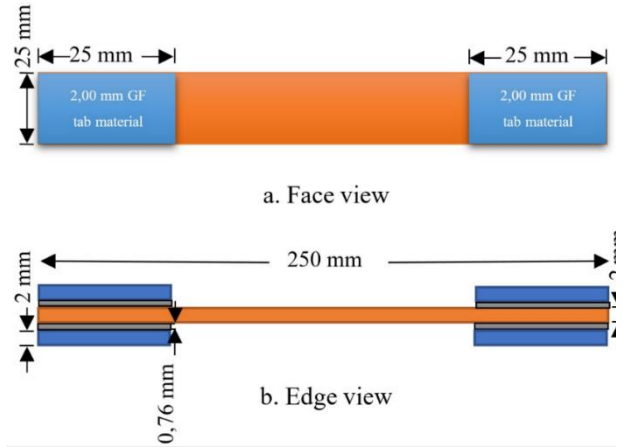
Figure 2. Tensile test specimen geometries according to ASTM D3039.
